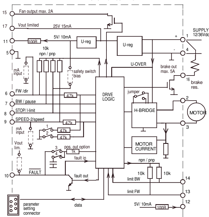
EM-247C PCB V.3 BLOCK DIAGRAM
