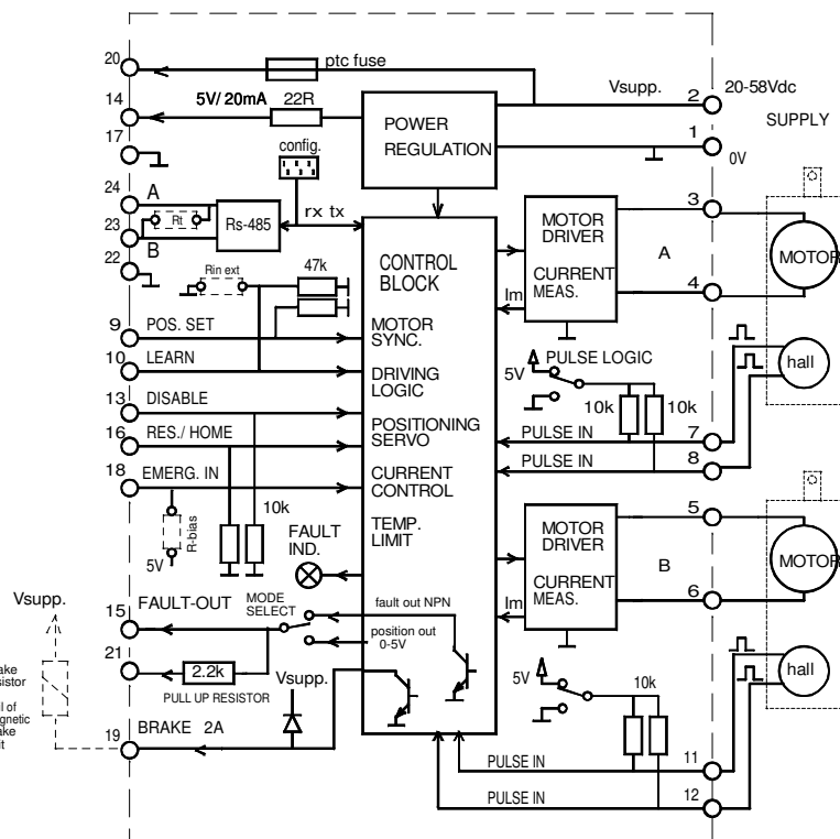
EM-339A-48V-SPF BLOCK DIAGRAM
